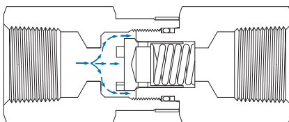
Valve in Tripped Position
