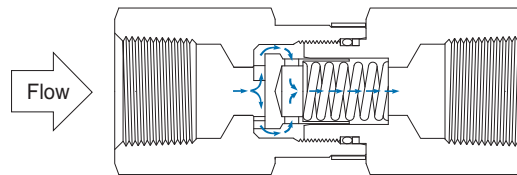
Valve in Open Position
